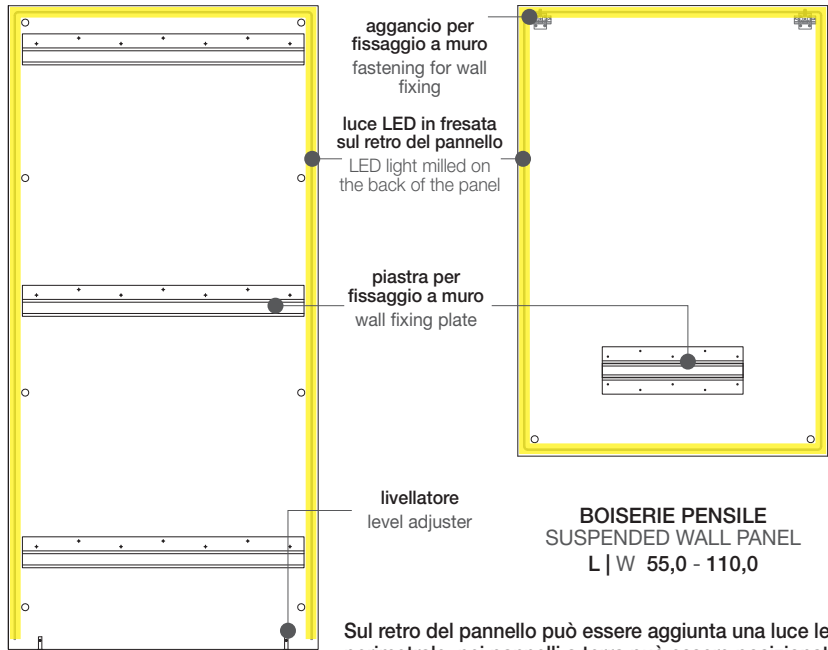
BOISERIE A TERRA FLOOR-STANDING WALL PANEL L | W 55,0 - 110,0
