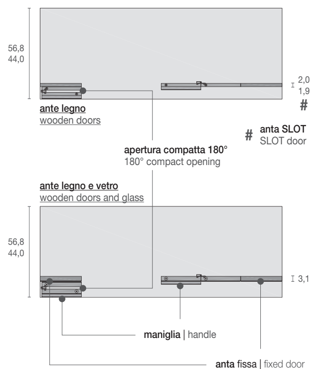
VISTA IN PIANTA PLAN VIEW
