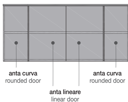
VISTA LATO ANTE DOORS SIDE VIEW
